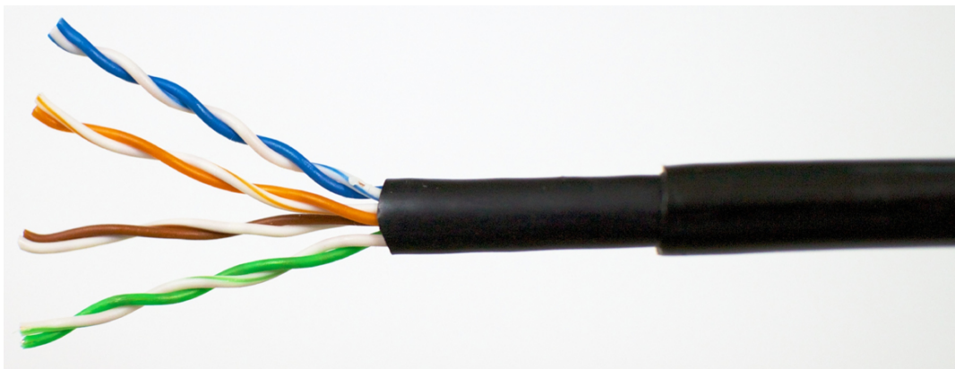
Twisted pair cable with four pairs, twisted at different rates. (Image by Thuansak Srilao © 123RF.com)
