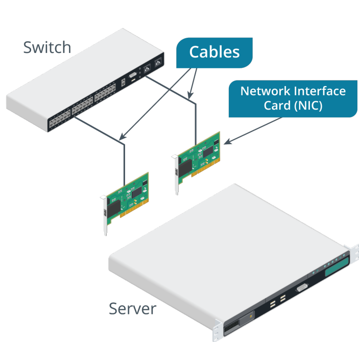
Server with redundant NICs plugged into one switch. (Images © 123RF.com)
