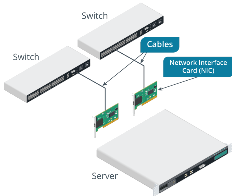
Server with redundant NICs plugged into redundant switches. (Images © 123RF.com)
