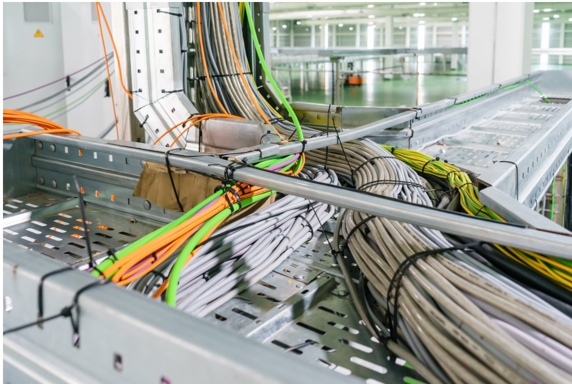
Overhead cable tray supporting bundles of cable. (Image by Pisit Khambubpha © 123RF.com)
