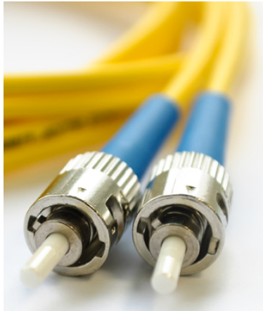
Two single-mode ST connectors. (Image by Aleh Datskevich © 123RF.com)
